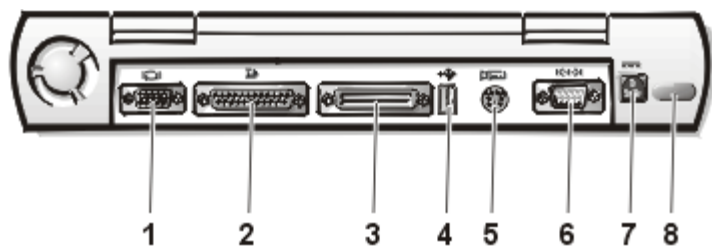
Figure 1. I/O Connectors
